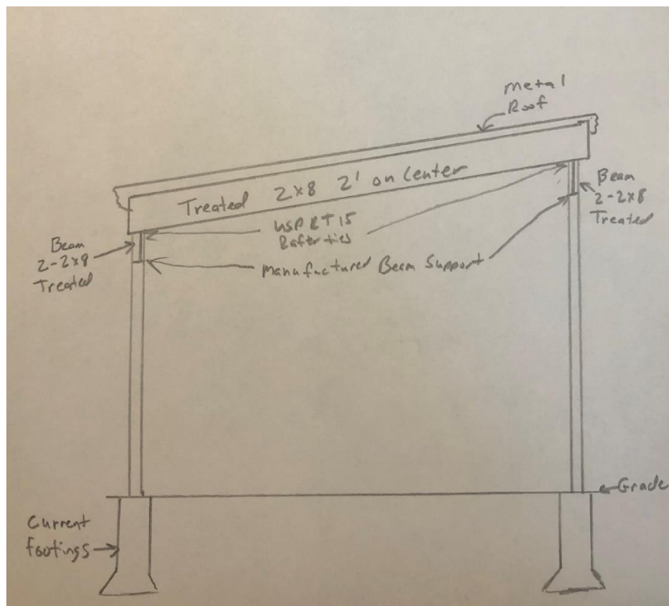
Plan for Dugout Roof:
