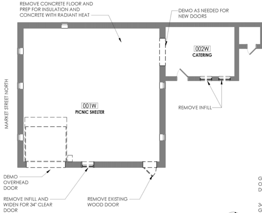
1 WORKSHOP DEMO PLAN P111 1/8" = 1'-0"
