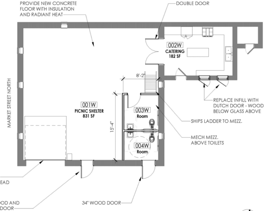
2 WORK SHOP GROUND LEVEL PLAN P111 1/8" = 1'-0"
