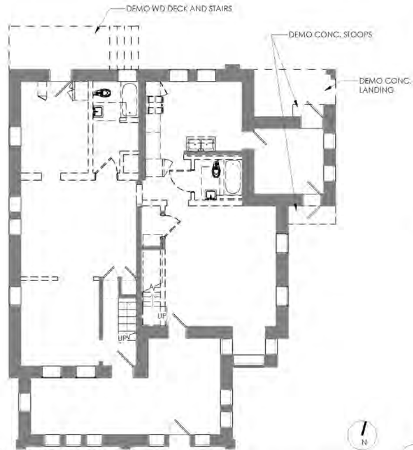
1 P101 GROUND FLOOR DEMO PLAN 1/8" = 1'-0"
