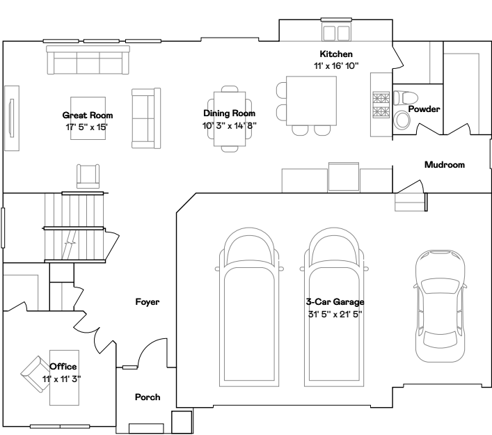
1st floor
