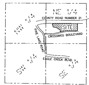
SECTION 14, TWP. 115, RGE. 22 LOCATION MAP NO SCALE
