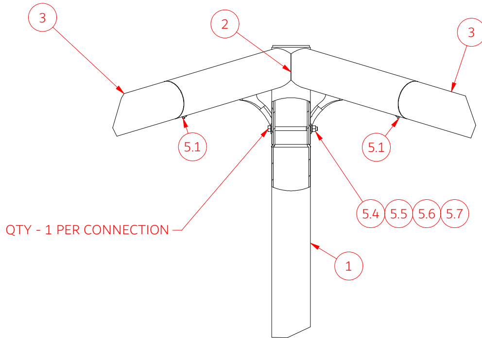
DETAIL R (BREAKOUT VIEW) CROSSPIECE-COLUMN FASTENING DETAIL SCALE 1"=1'
