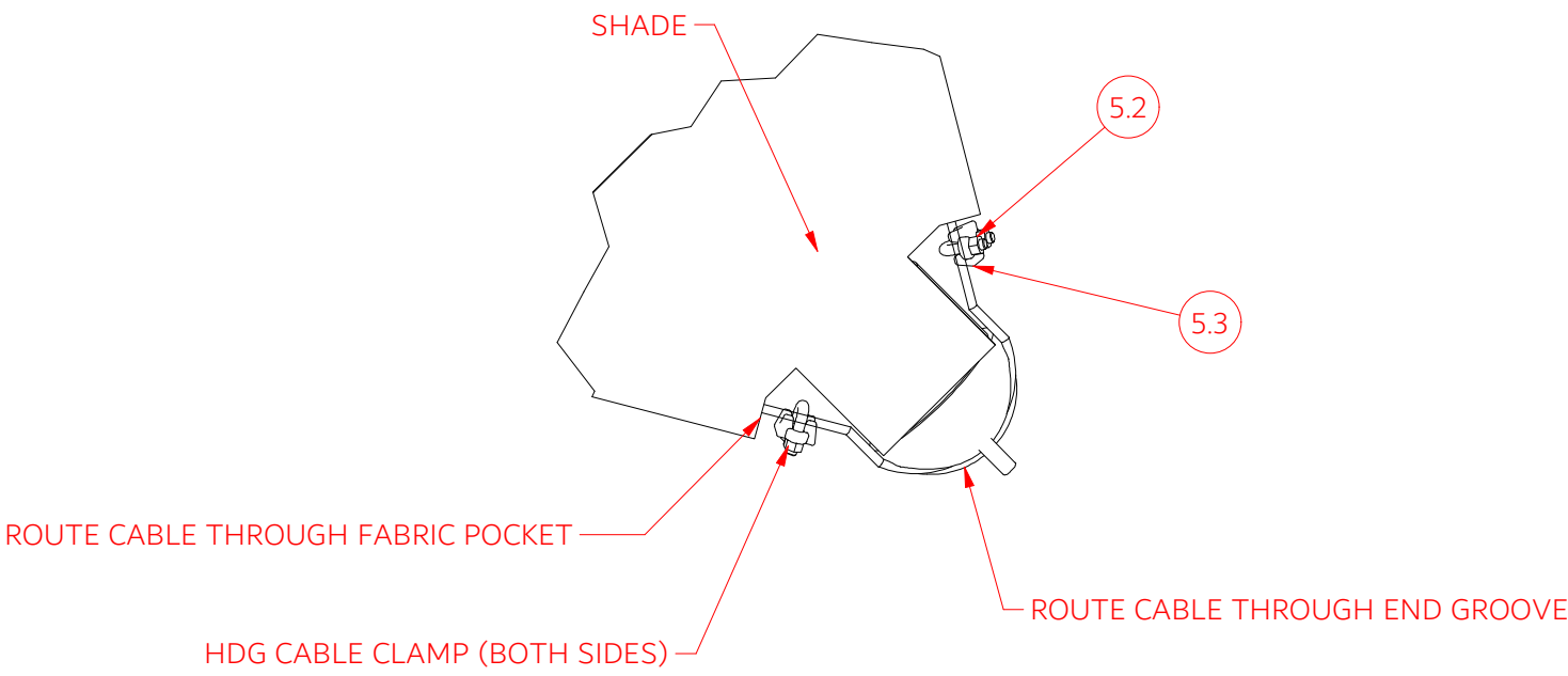
DETAIL P SHADE-CABLE CONNECTION SCALE 1/6
