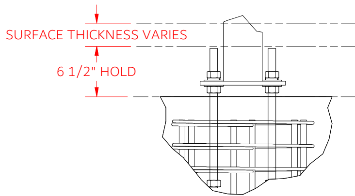
DETAIL M SURFACING NOTES SCALE 1"=1'
