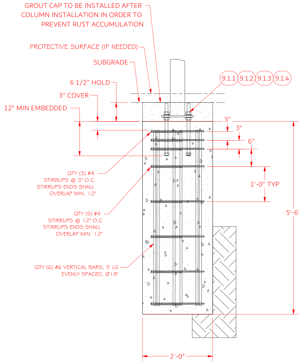
DETAIL H PIER FOUNDATION SCALE 3/4"=1'-0"
