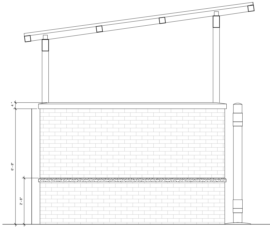
ELEVATION @ TRASH ENCLOSURE
