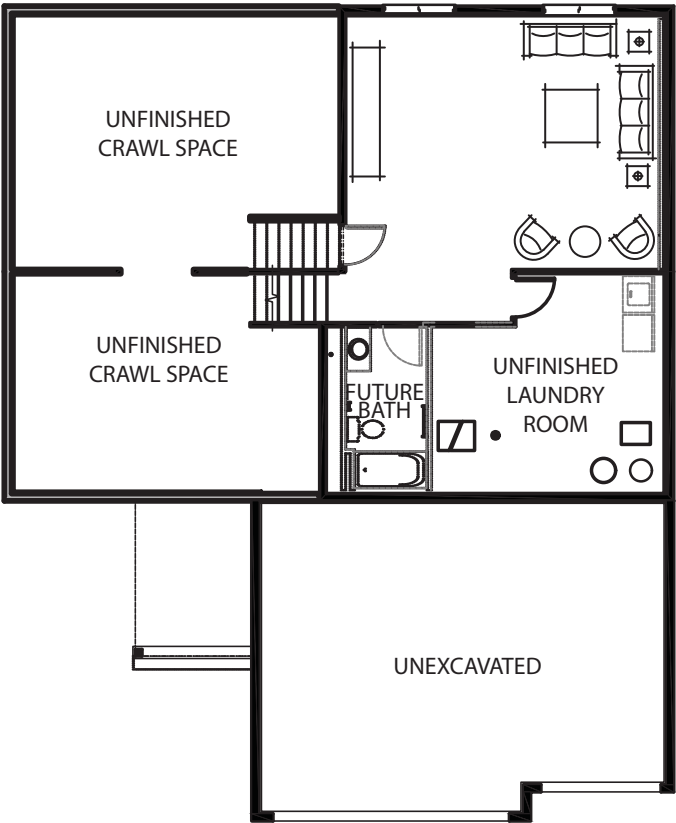
LOWER LEVEL
