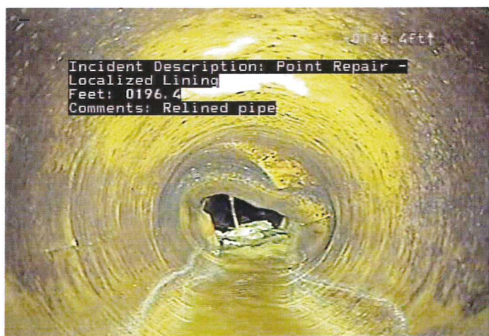
RPL - Point Repair - Localized Lining @ 194.3 ft. Relined pipe
